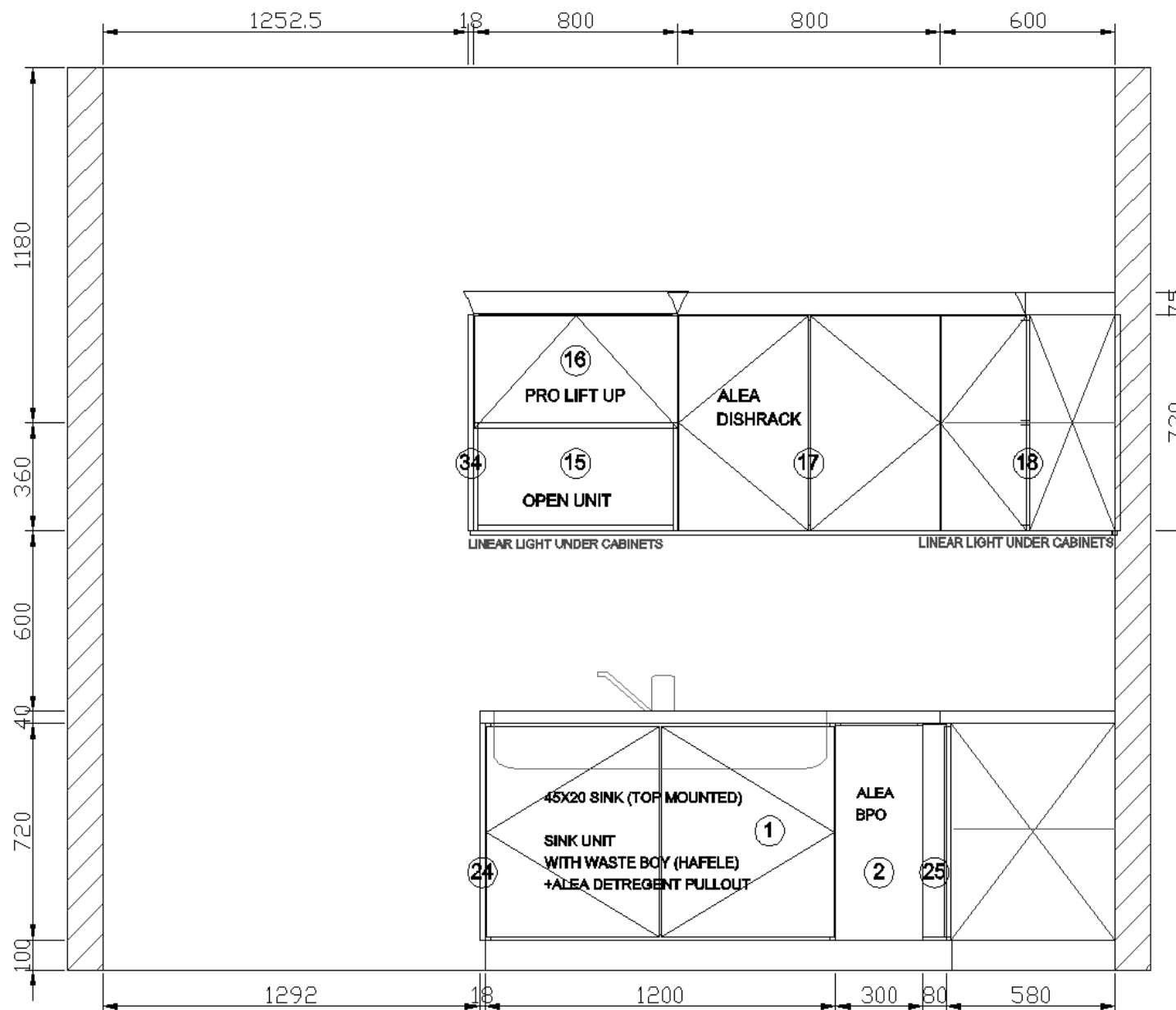
C View elevation drawing
