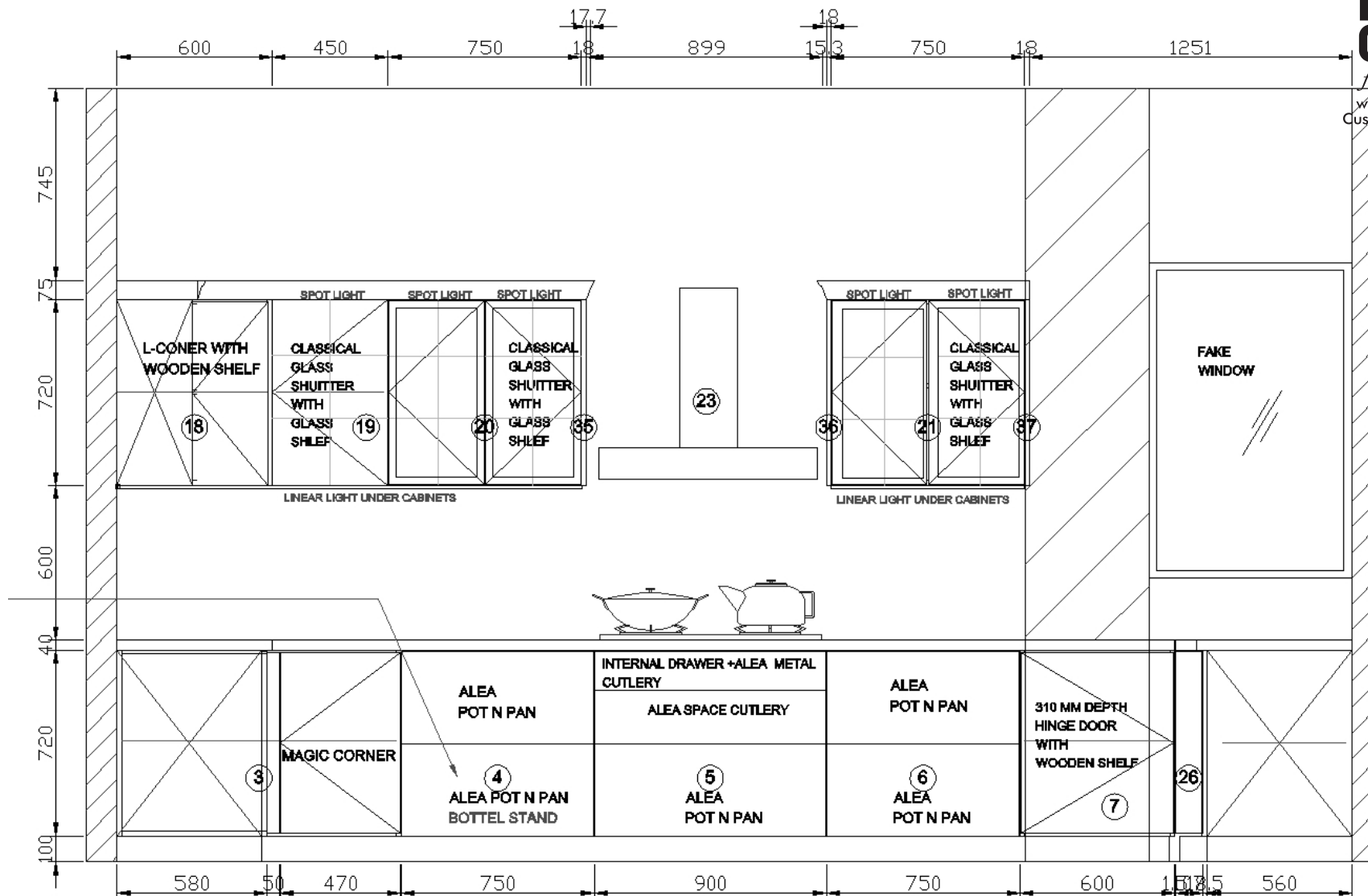
A View elevation drawing
