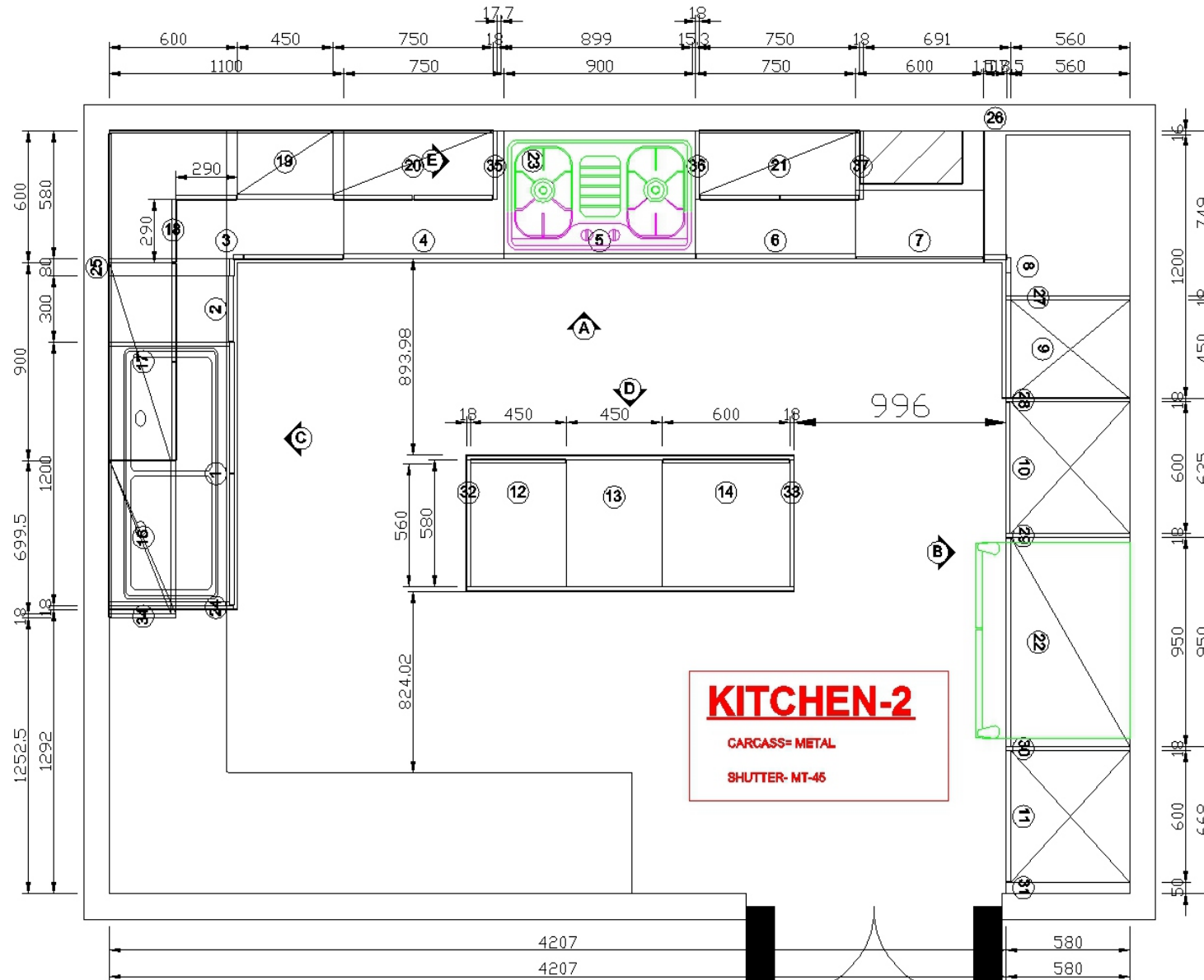
Plan drawing
